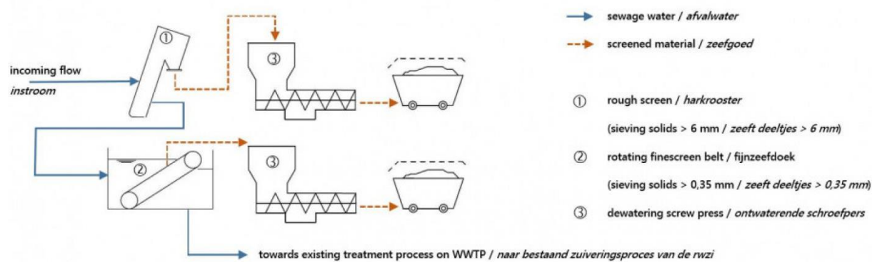
Figure 8-14: The process of harvesting cellulosic screenings
