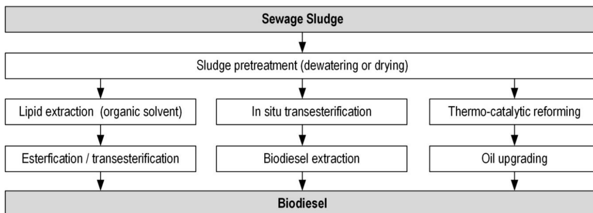
Figure 4-3: Schematic presentation of Biodiesel production routes based on sewage sludge that are in the center of ongoing research
