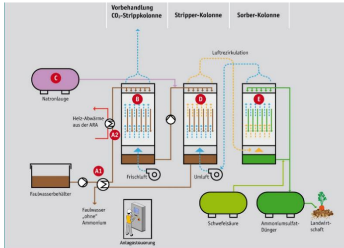
Figure 8-12: Process diagram of ammonia stripping in the WWTP Kloten/ Opfikon (Liebi, 2014)
