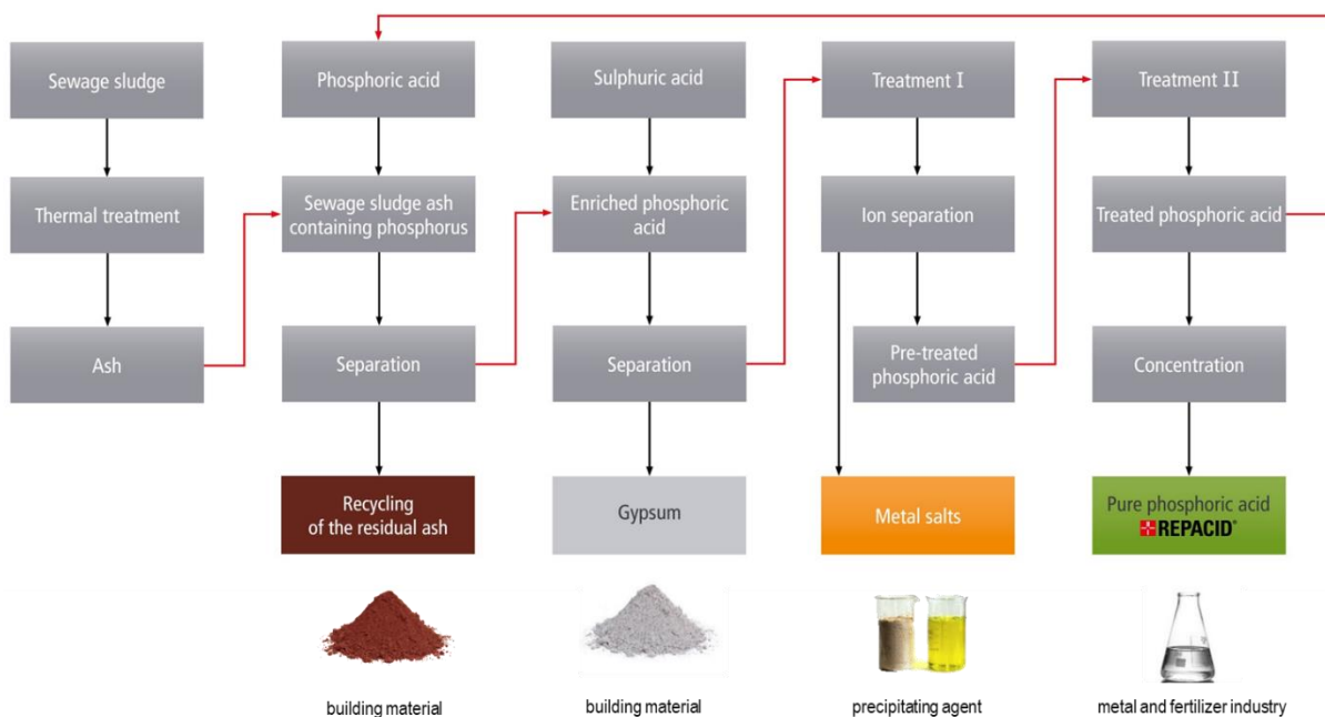
Figure 8-2 Flow sheet of TetraPhos™-process
