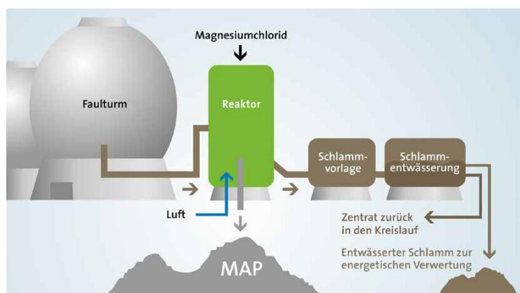
Figure 8-11: Process for obtaining MAP (Product sheet MAP)
